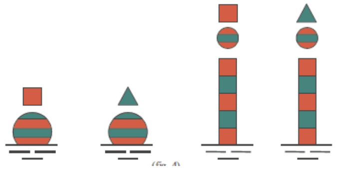
Cevni buoyage & markings
